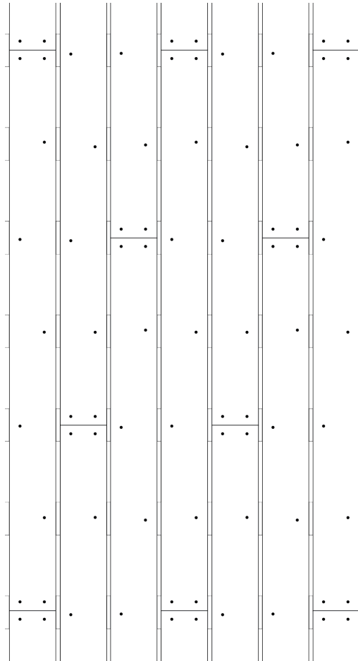
Decking nailing pattern
